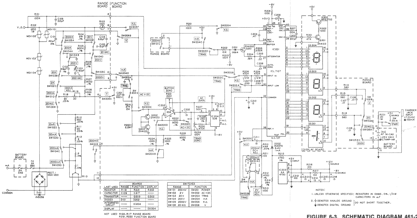
FIGURE 6-3. SCHEMATIC DIAGRAM 461-2R
